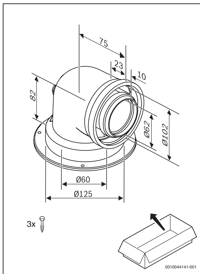
2 Ø 60/100: 7738113793
