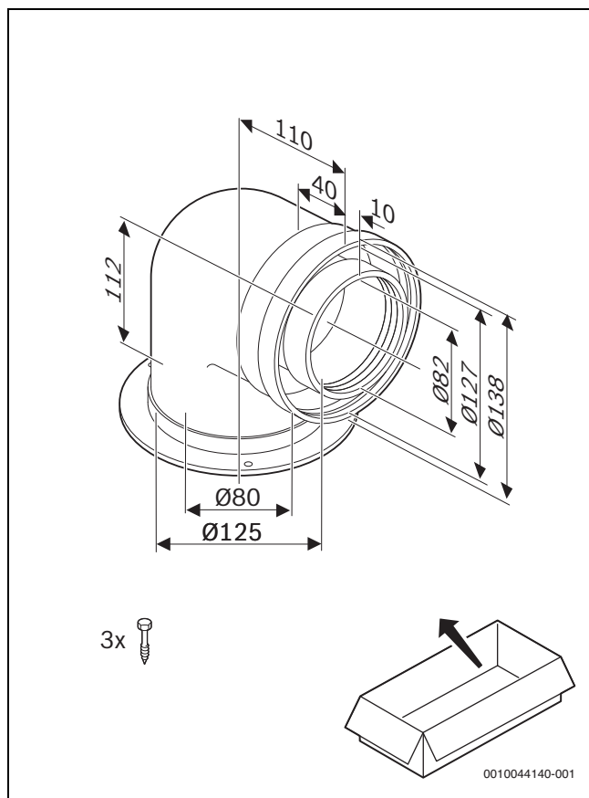
3 Ø 80/125: 7738112717
