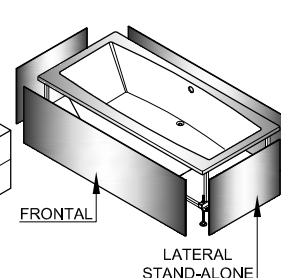
STAND-ALONE APPLICATION (Frontal panel+lateral stand-alone panel)
