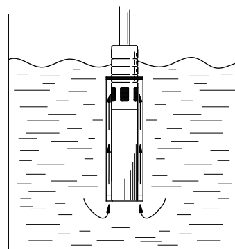
Fig. 36 Flow sleeve function
