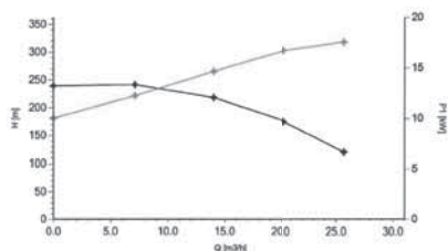
Measured values for tested pump
