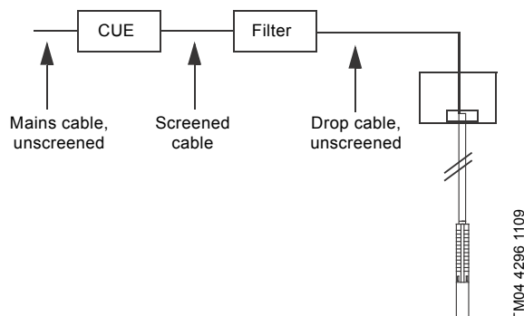
Fig. 26 Example of installation in EMC-insensitive sites
