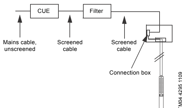
Fig. 27 Example of installation in EMC-sensitive sites
