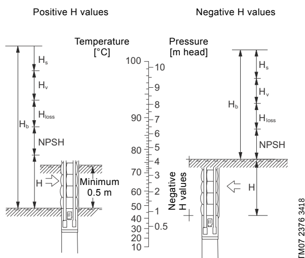
Fig. 20 Installation depth
