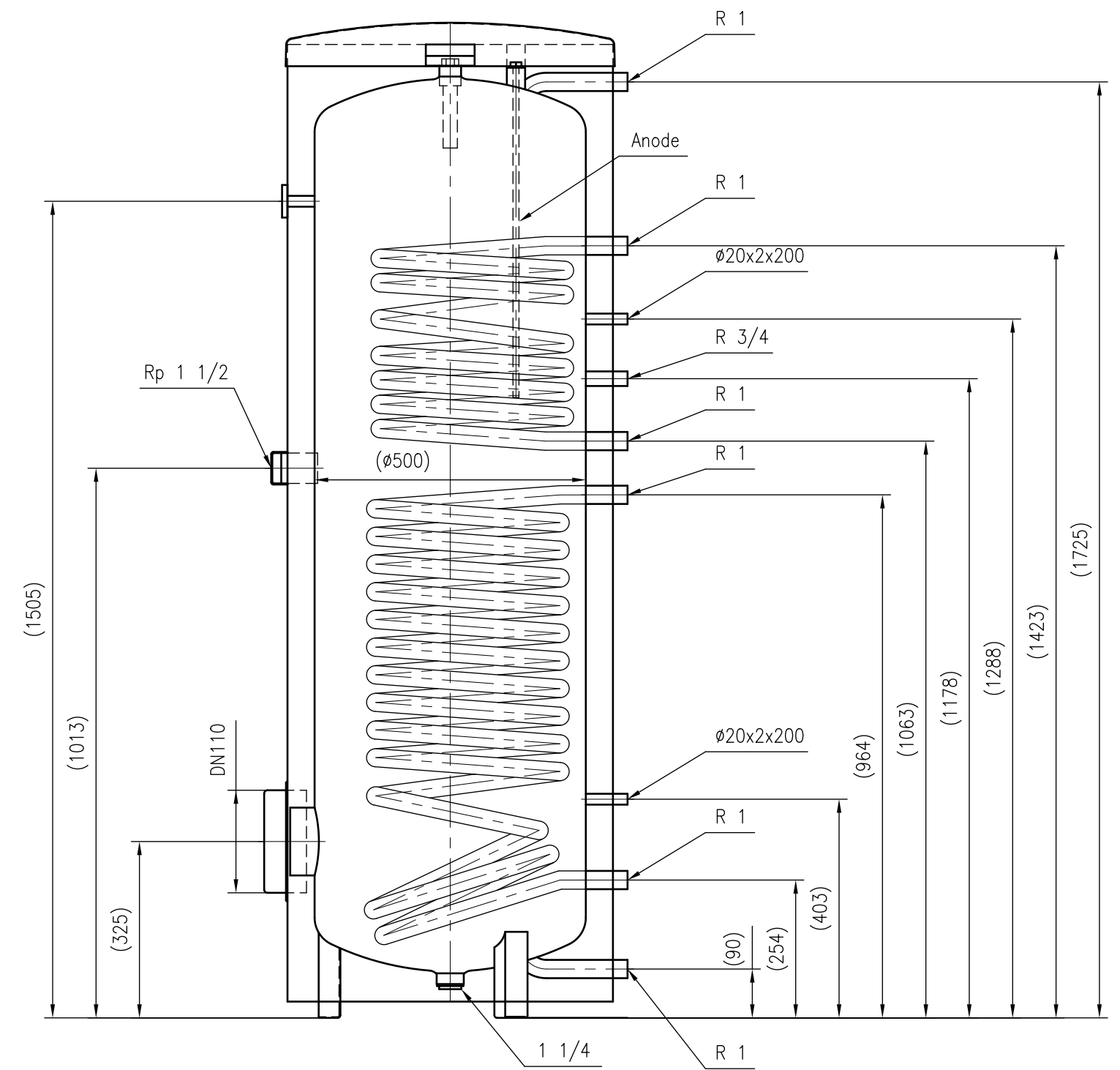
Side view
