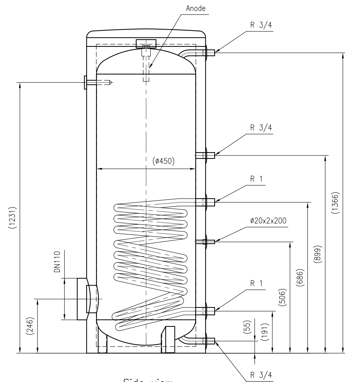
Side view
