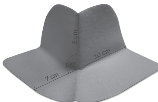
ECODRY50 CORNEROUT
