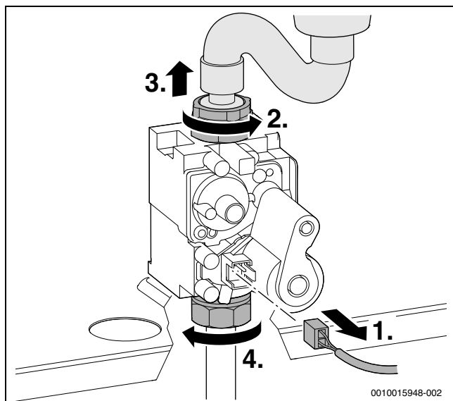
Fig. 59 Retirar as fichas e soltar as porcas de capa
