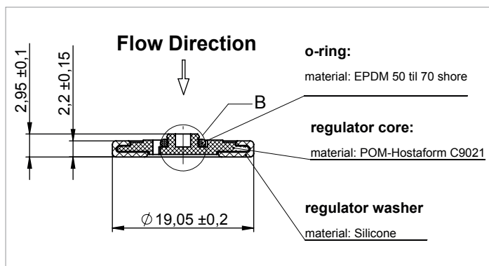
PCW-01 1/2" washer regulator
