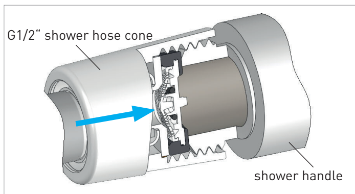
Recommended mounting position for shower handles
